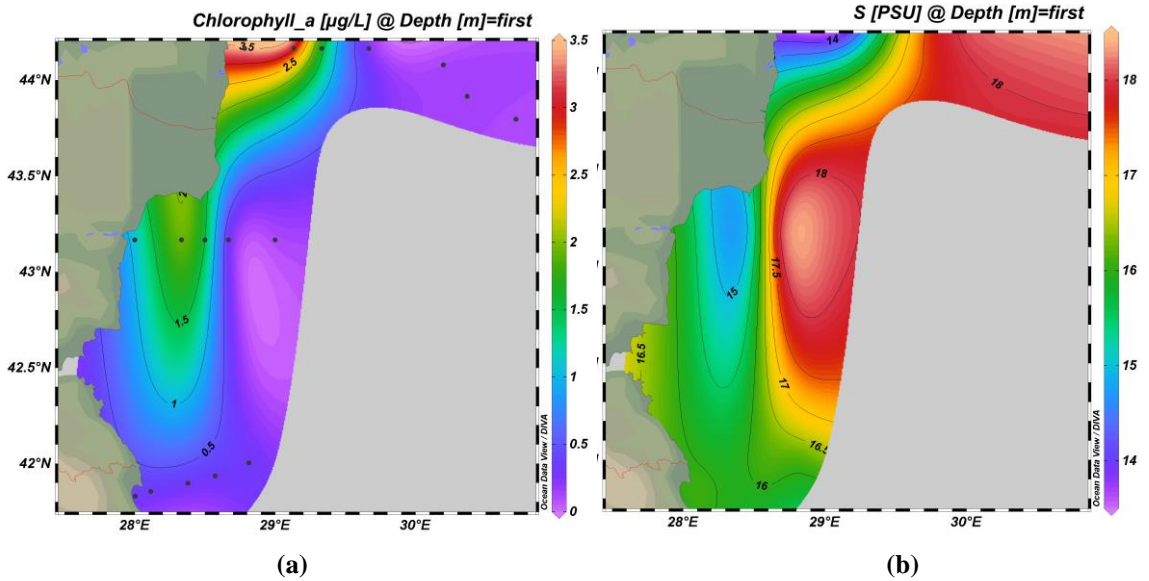
Fig. 7. Chlorophyll \alpha (a) and salinity (b) surface distributions - Western Black Sea, July 2013
