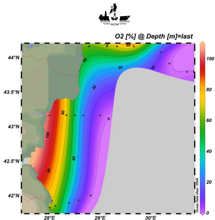
Fig. 8. Bottom dissolved oxygen saturation distribution - Western Black Sea, July 2013
