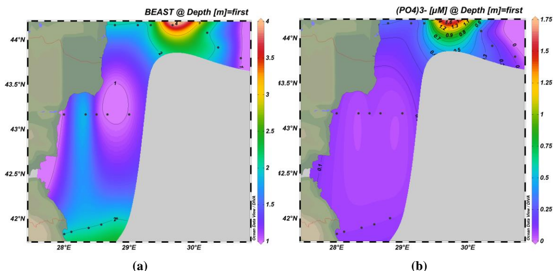
Fig. 2. (a) BEAST and phosphate (b) surface distribution - Western Black Sea, July 2013
